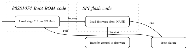
Fig. 1. Crucial MX300 boot process.
