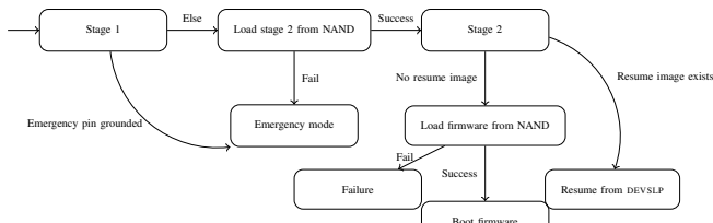
Fig. 4. Samsung 850 EVO boot process.
