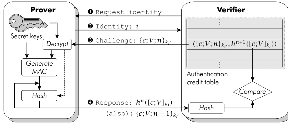
Figure2. Authentication protocol using OTP
