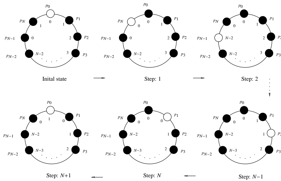
Fig. 4.1: A counter-example: a ring with K = N - 1
