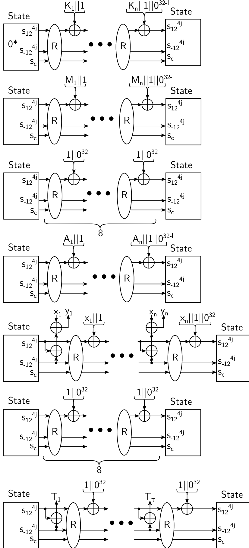
Figure 13: Subterranean-Subauthenticated Encryption (SAE), only encryption is illustrated.
